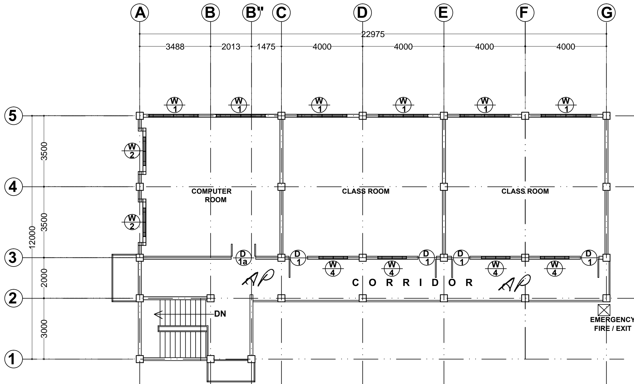
1 SECOND FLOOR PLAN SCALE: NTS 0 500 1m 2m
