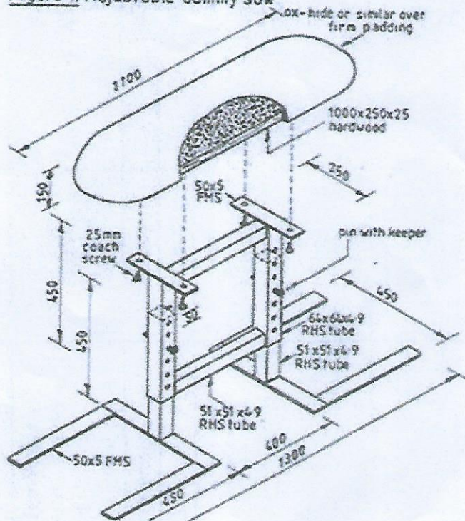
Figure 1. Adjustable dummy sow
