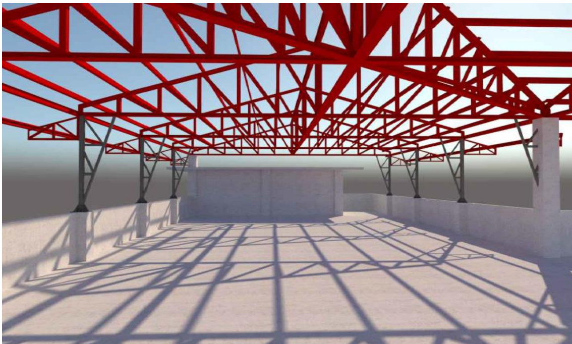
PERSPECTIVE VIEW
