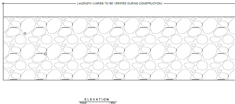
DETAIL OF PROPOSED DRY RIPRAP SCALE: 1:30 meters
