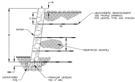
TYPICAL SECTION-REINFORCED GEOGRID SCALE: NTS
