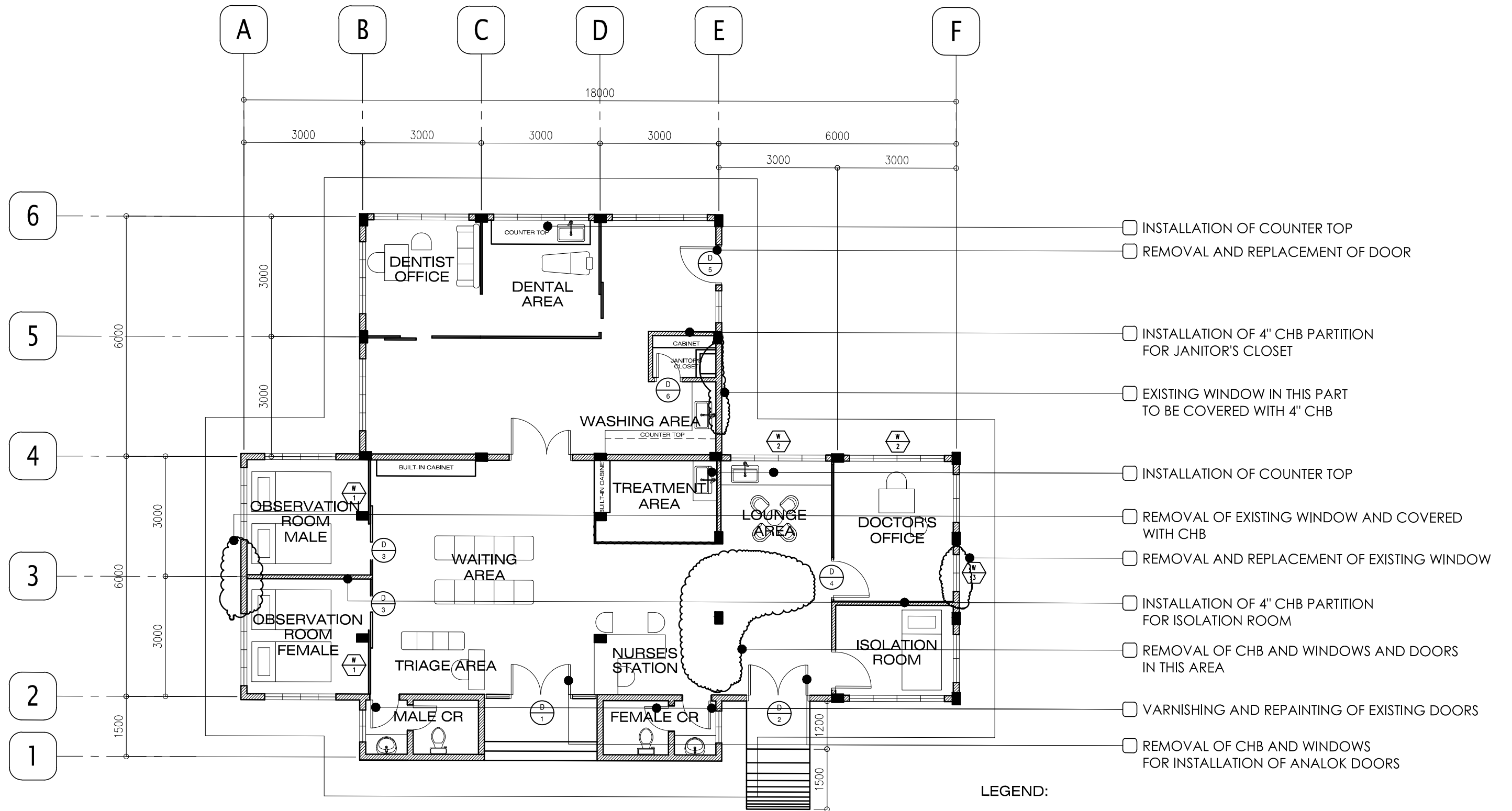
1 A 2 FLOOR PLAN SCALE 1:100 m.
