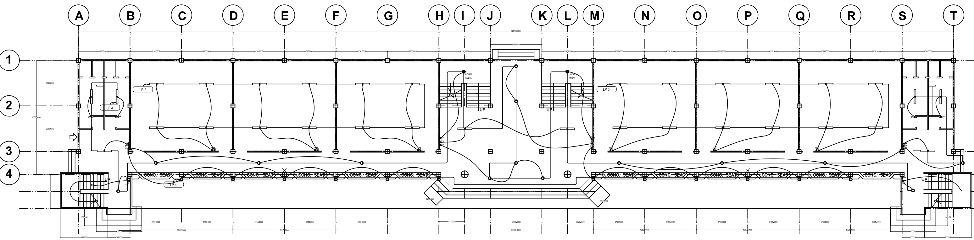
1 GROUND FLOOR LIGHTING LAYOUT SCALE 1:100 m.
