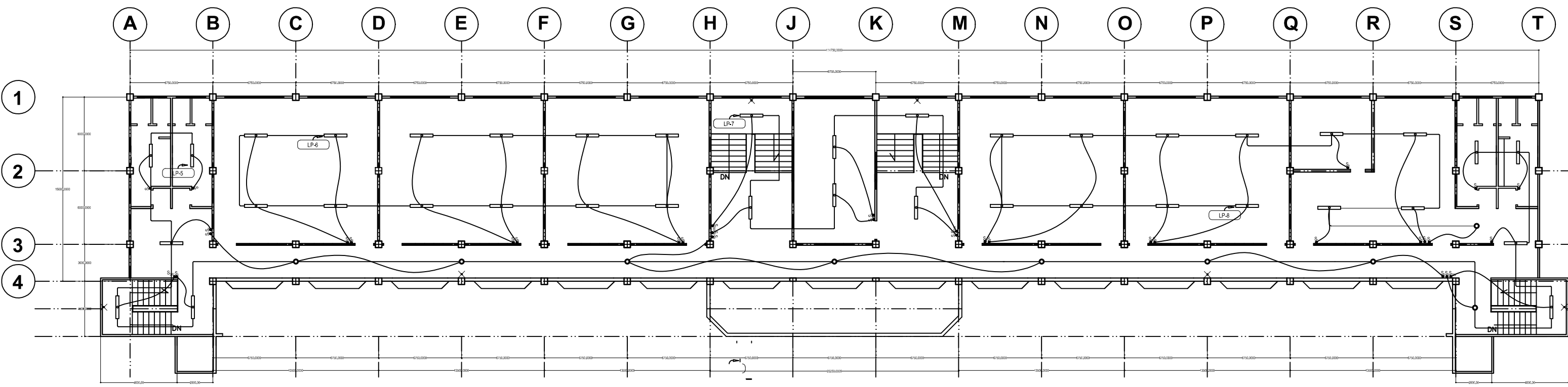
1 SECOND FLOOR LIGHTING LAYOUT E 2 SCALE 1:100 m.
