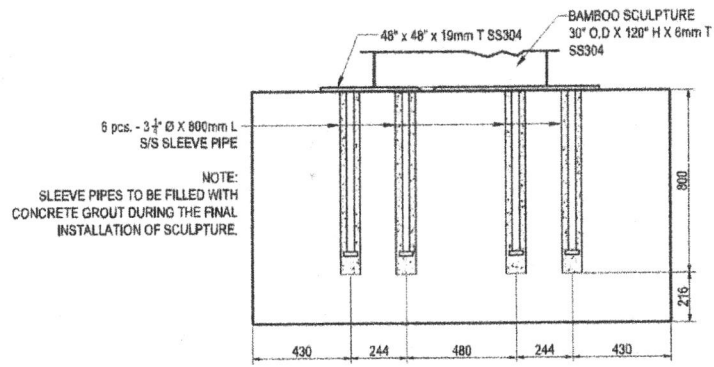
S/S SLEEVE PIPES LAYOUT DETAIL
