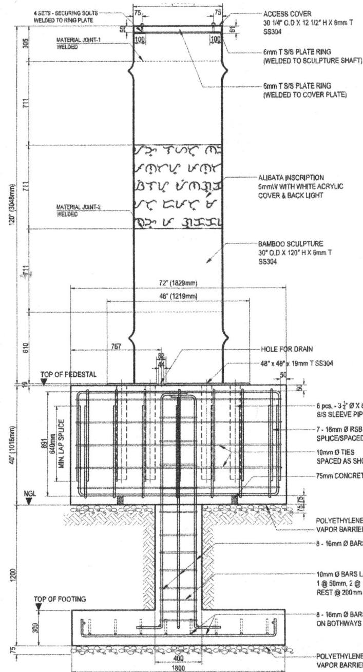
SECTION
