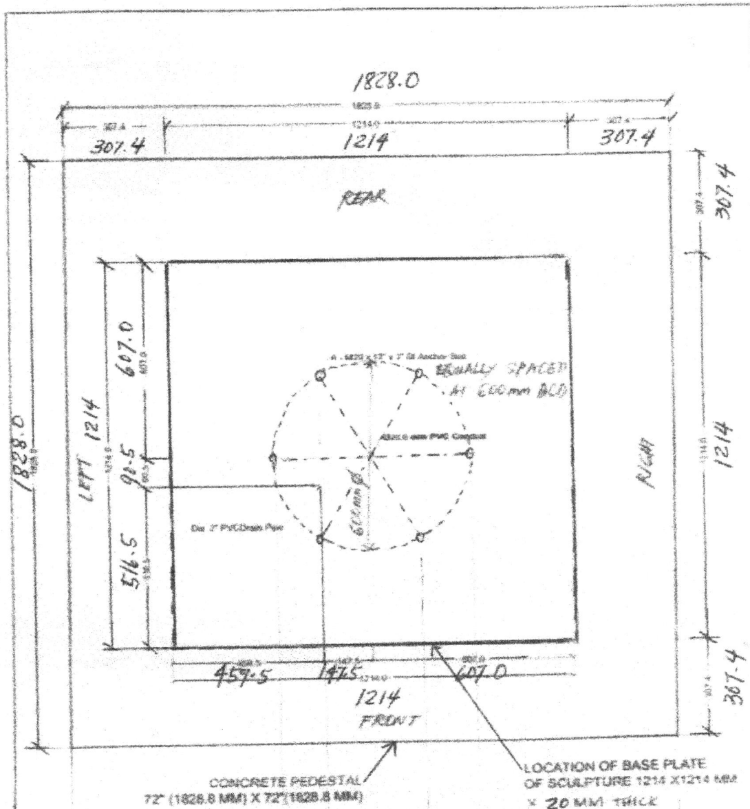
TOP VIEW
