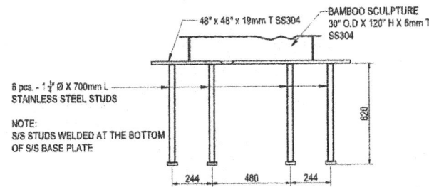
S/S STUDS LAYOUT DETAIL
