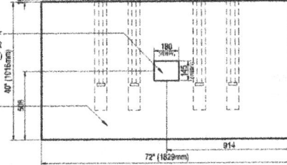
REAR ELEVATION
