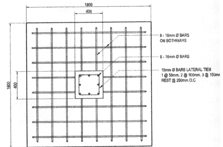
PLAN (FOOTING)
