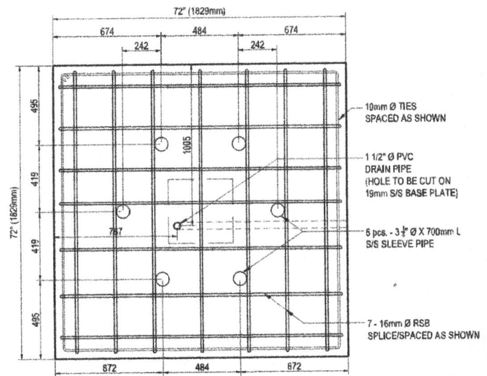
PLAN (PEDESTAL)
